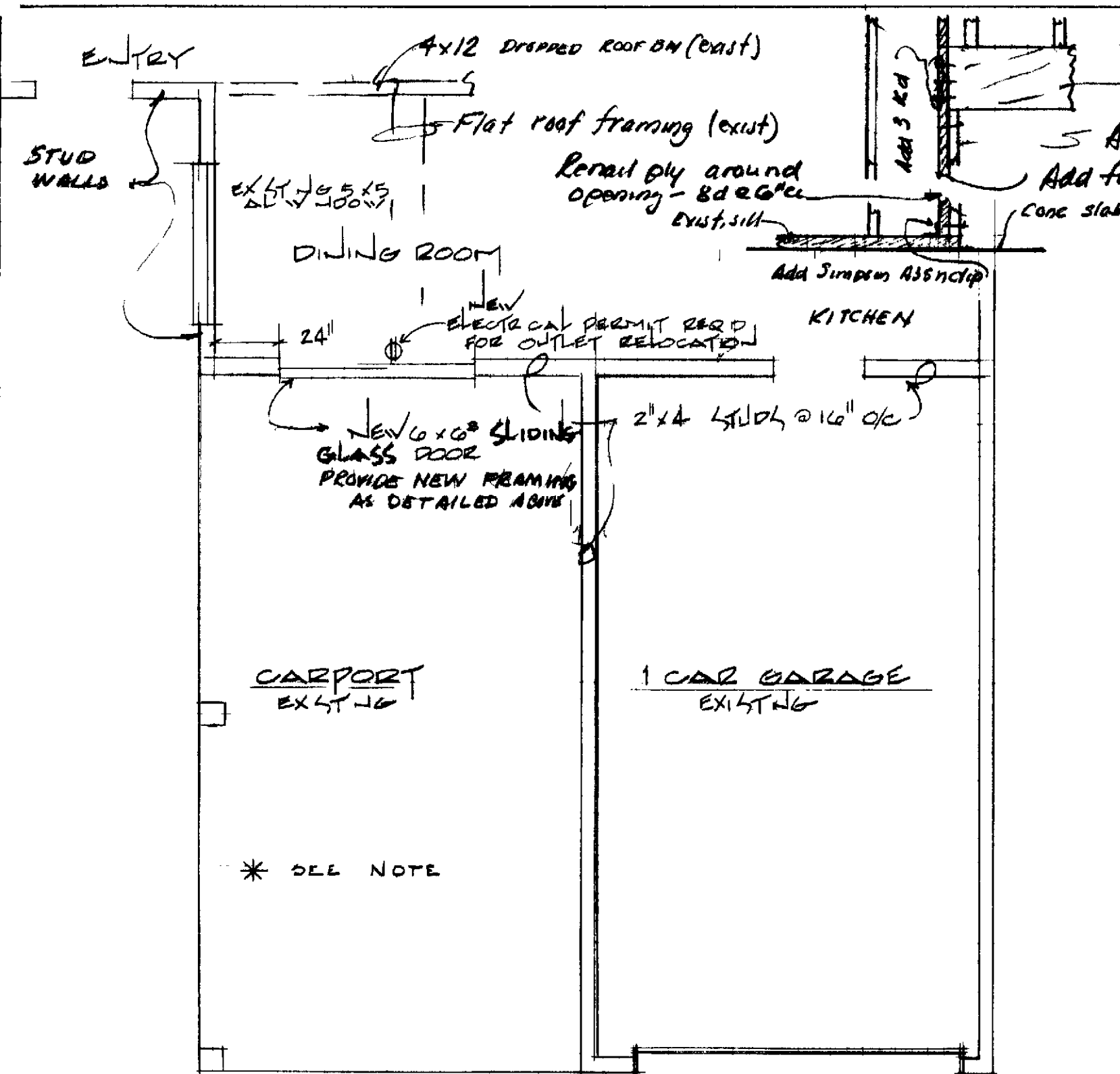
PARTIAL PLAN VIEW 1/4" SCALE
